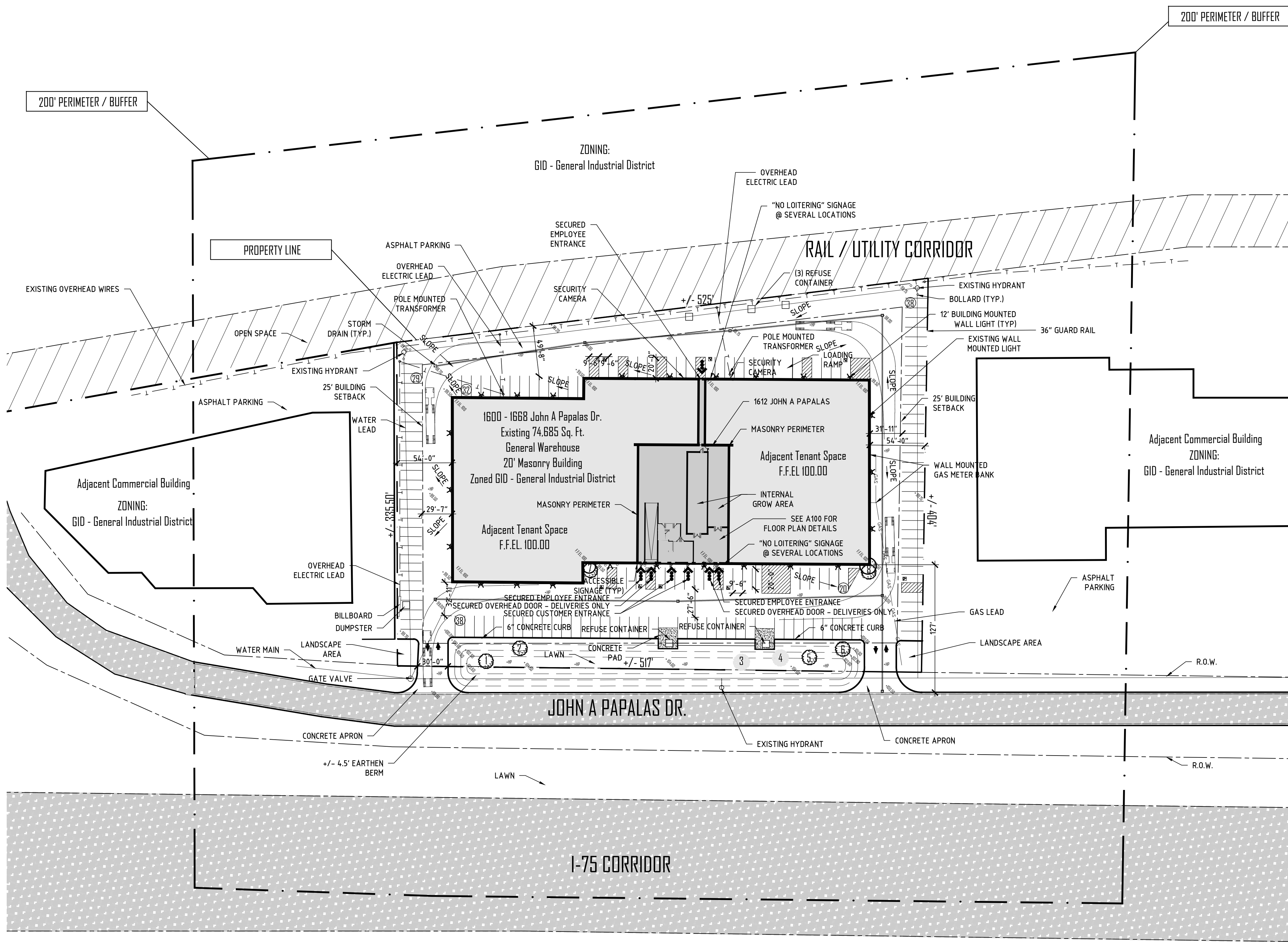
1 Site Plan 1"=60'
